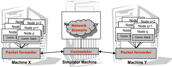
Figure 1: High-Level Architecture of CyberVAN
